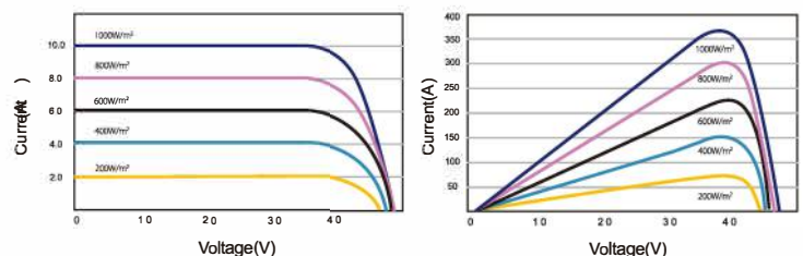
Current-Voltage & Power-Voltage(390W)
